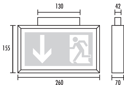
KD Decke / ceiling
